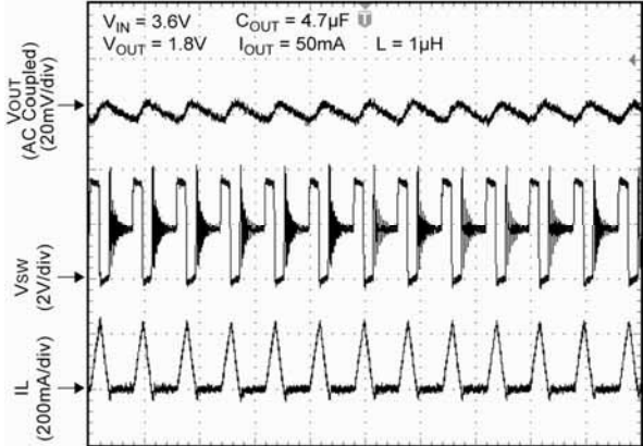
Switching Waveform - Discontinuous Mode
