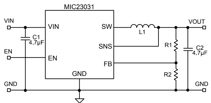
Figure 1. MIC23031-AYMT Schematic
