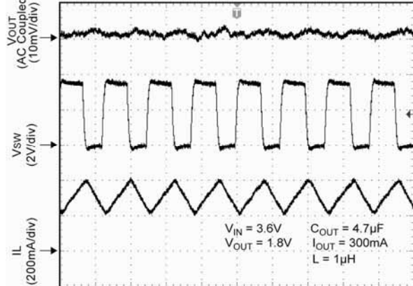
Switching Waveform - Continuous Mode
