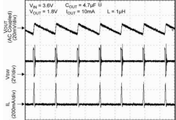
Switching Waveform - Discontinuous Mode
